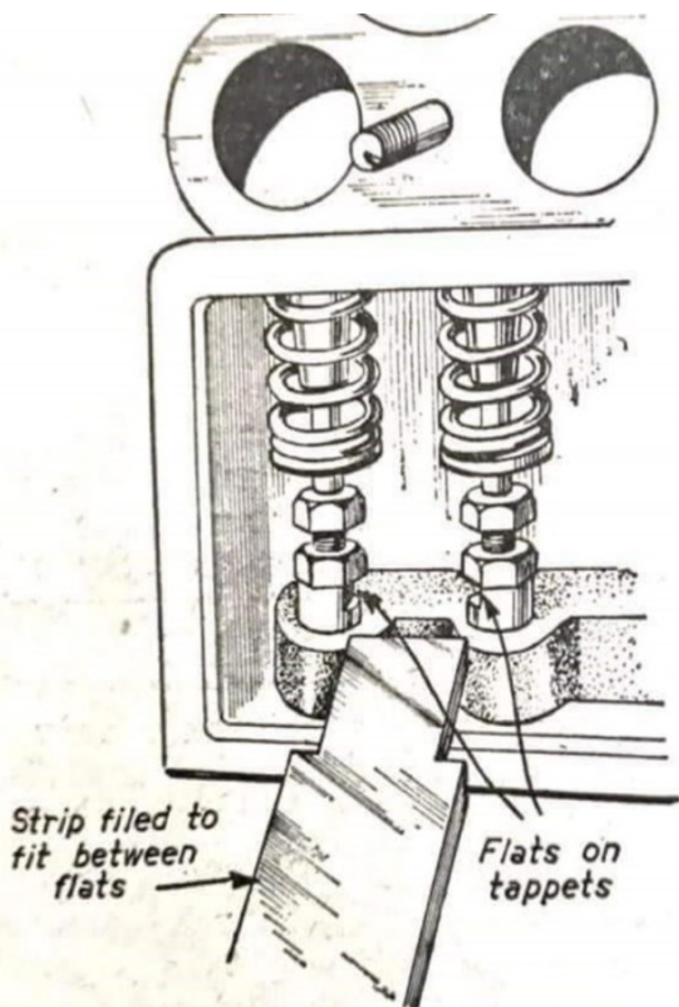
Fig. 10. —Instead of using three spanners when adjusting the tappets, the tappet can be prevented from rotating by filing a strip of metal until it will just fit between two adjacent flats, as shown. Two spanners can then be used on the lock-nut and tappet screw in the usual way.
