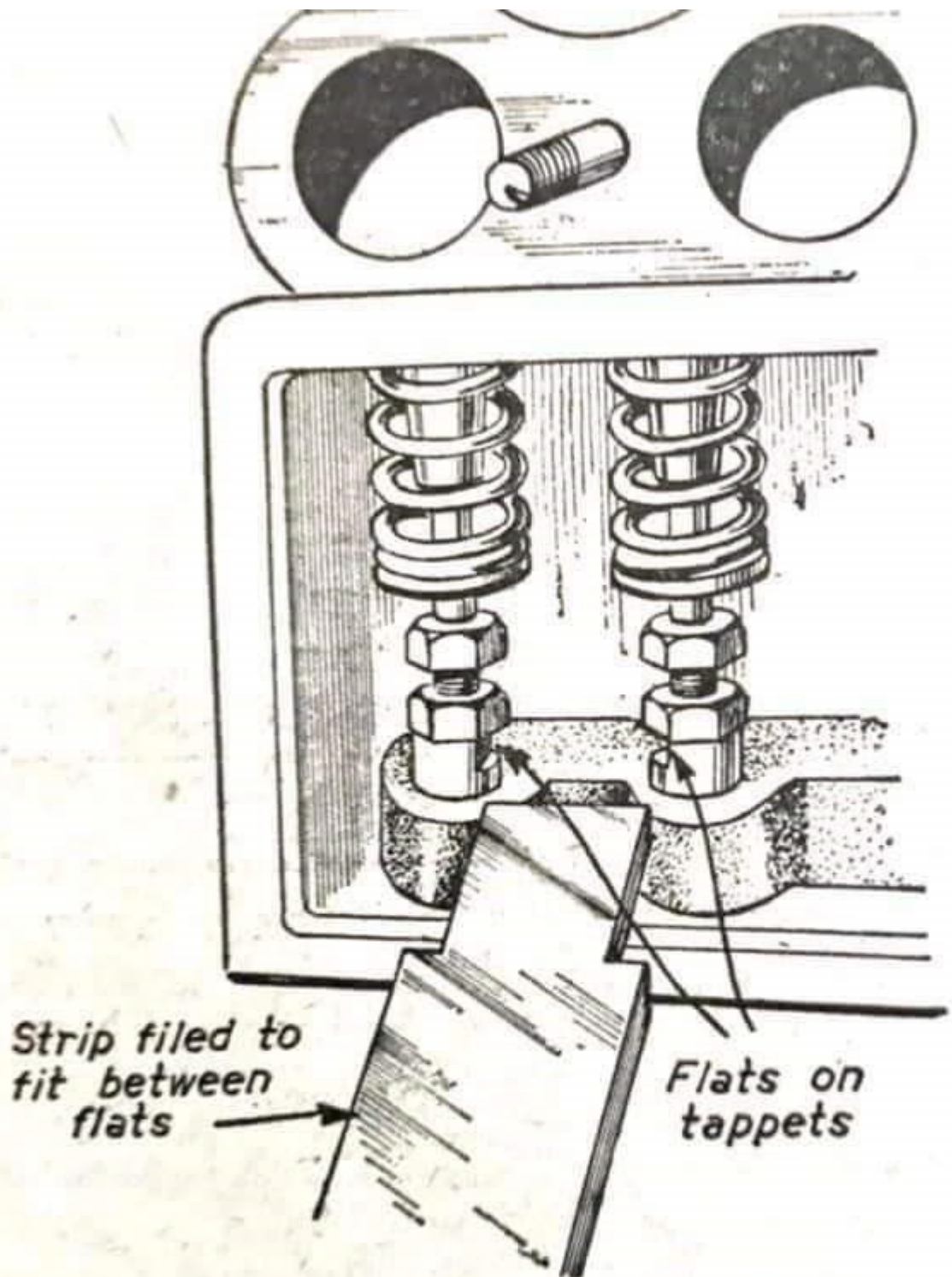
Fig. 10. —Instead of using three spanners when adjusting the tappets, the tappet can be prevented from rotating by filing a strip of metal until it will just fit between two adjacent flats, as shown. Two spanners can then be used on the lock-nut and tappet screw in the usual way.
