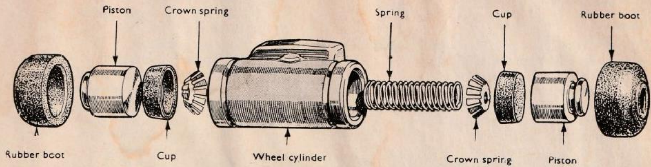
Fig 4—The component parts of a wheel cylinder, 8 hp and 10 hp.
