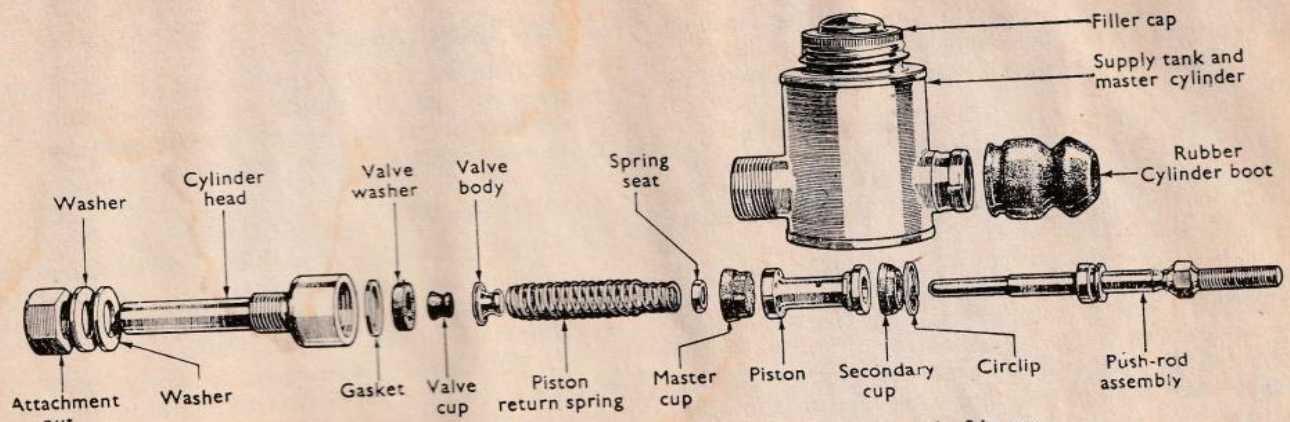
Fig 2—The component parts of the master cylinder and supply tank unit on the 8 hp car.
